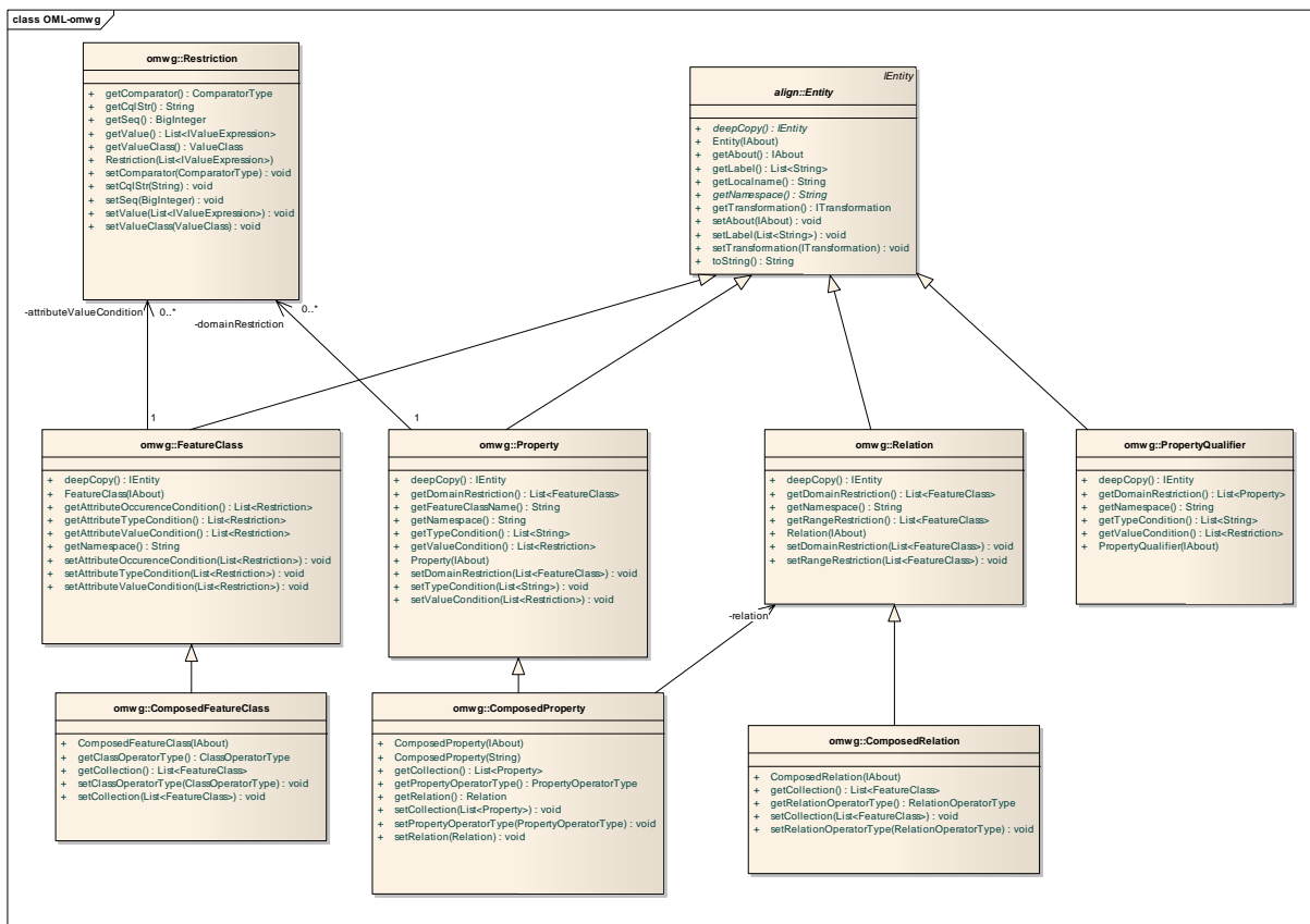
Figure 3: The classes of the omwg package of the gOML
