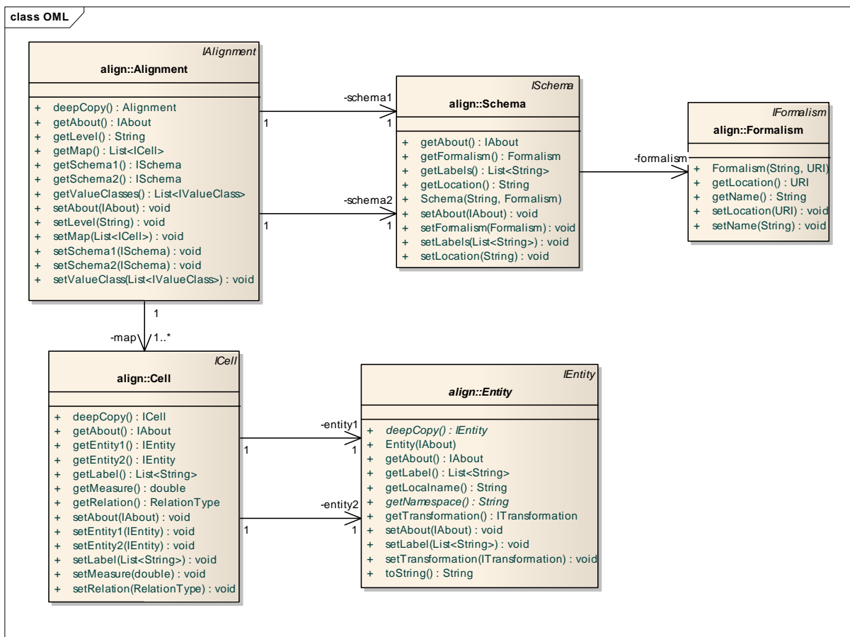
Figure 2: The classes of the align package of the gOML
