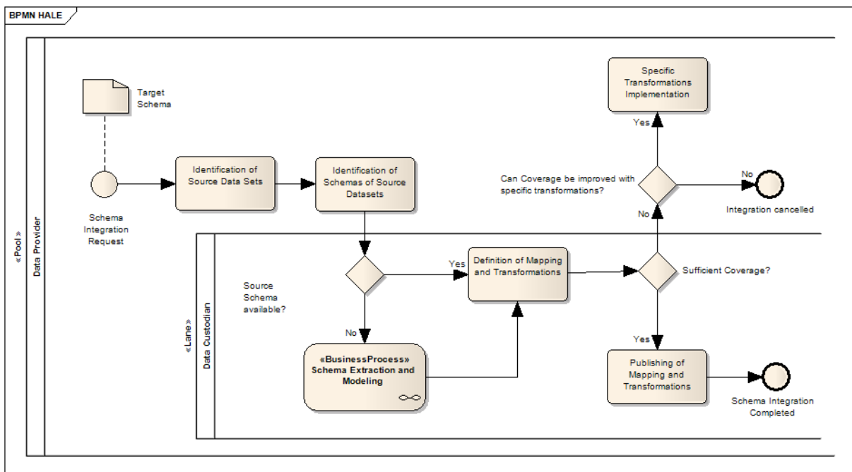
Figure 1: The overall business process associated with the schema specification mapping activities
